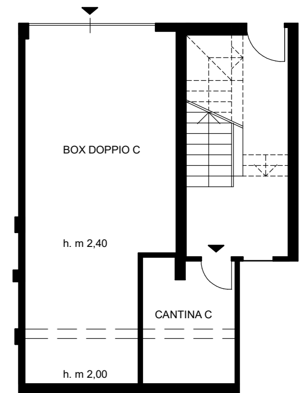
PIANO INTERRATO
